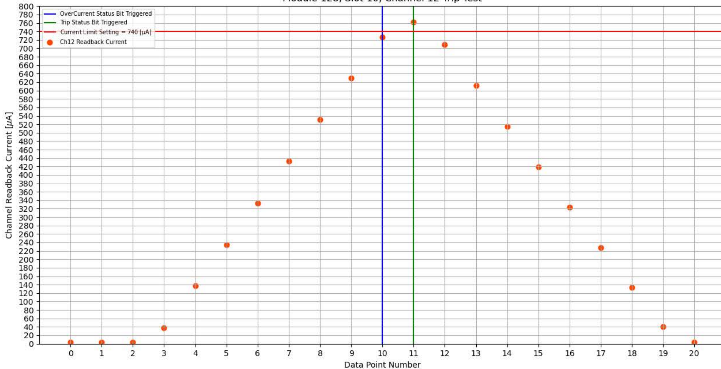
Module 128, Slot 10, Channel 12 Trip Test
