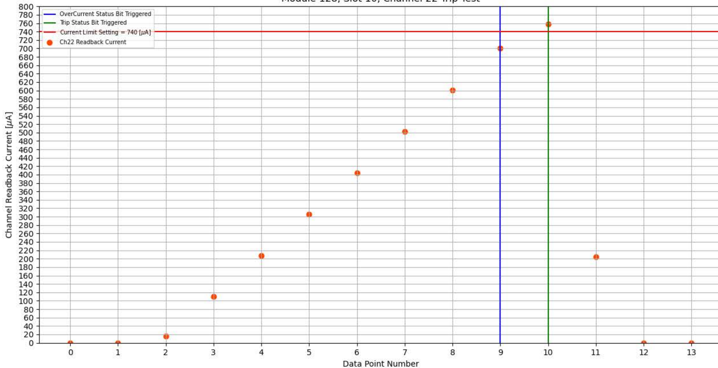
Module 128, Slot 10, Channel 22 Trip Test
