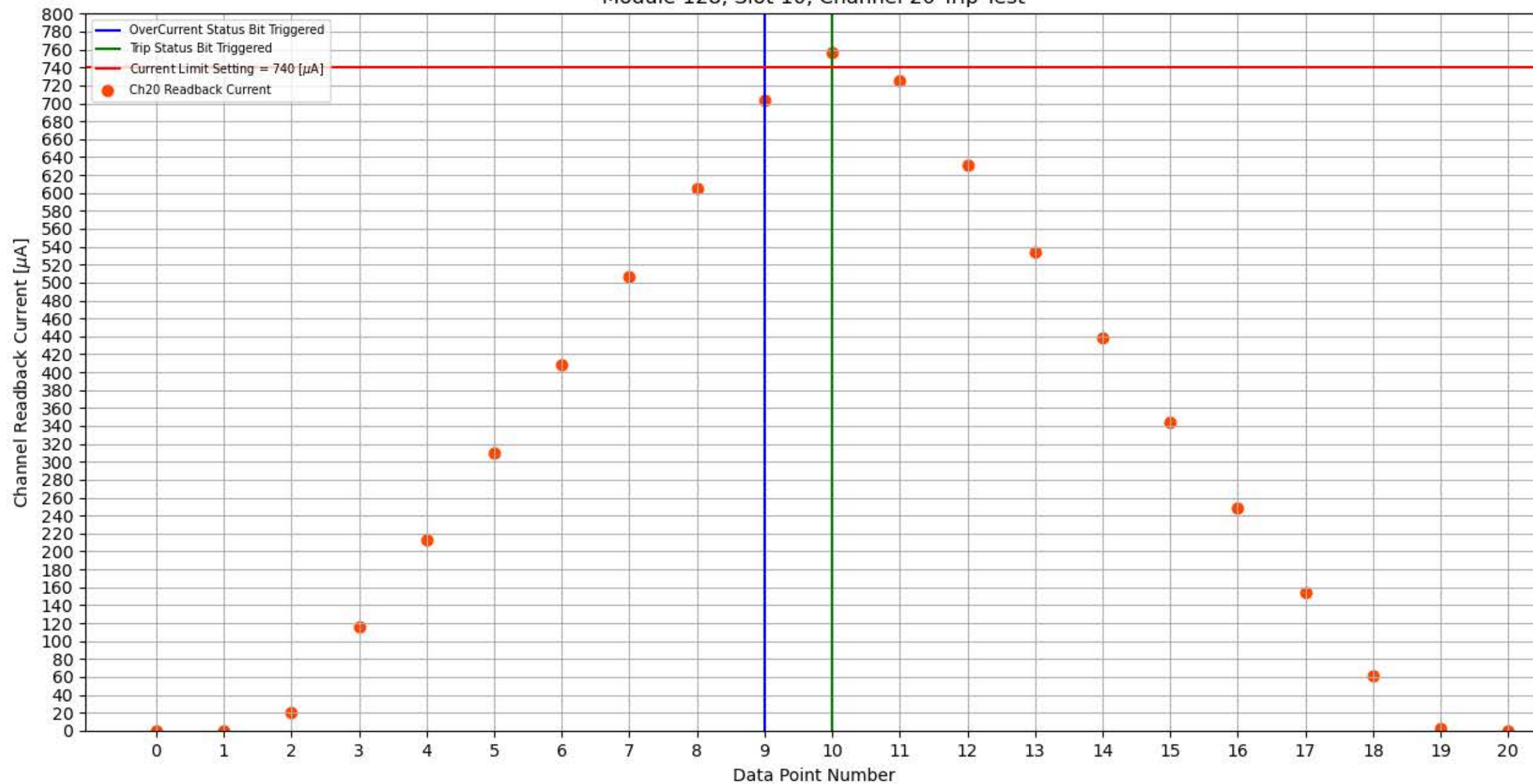
Module 128, Slot 10, Channel 20 Trip Test
