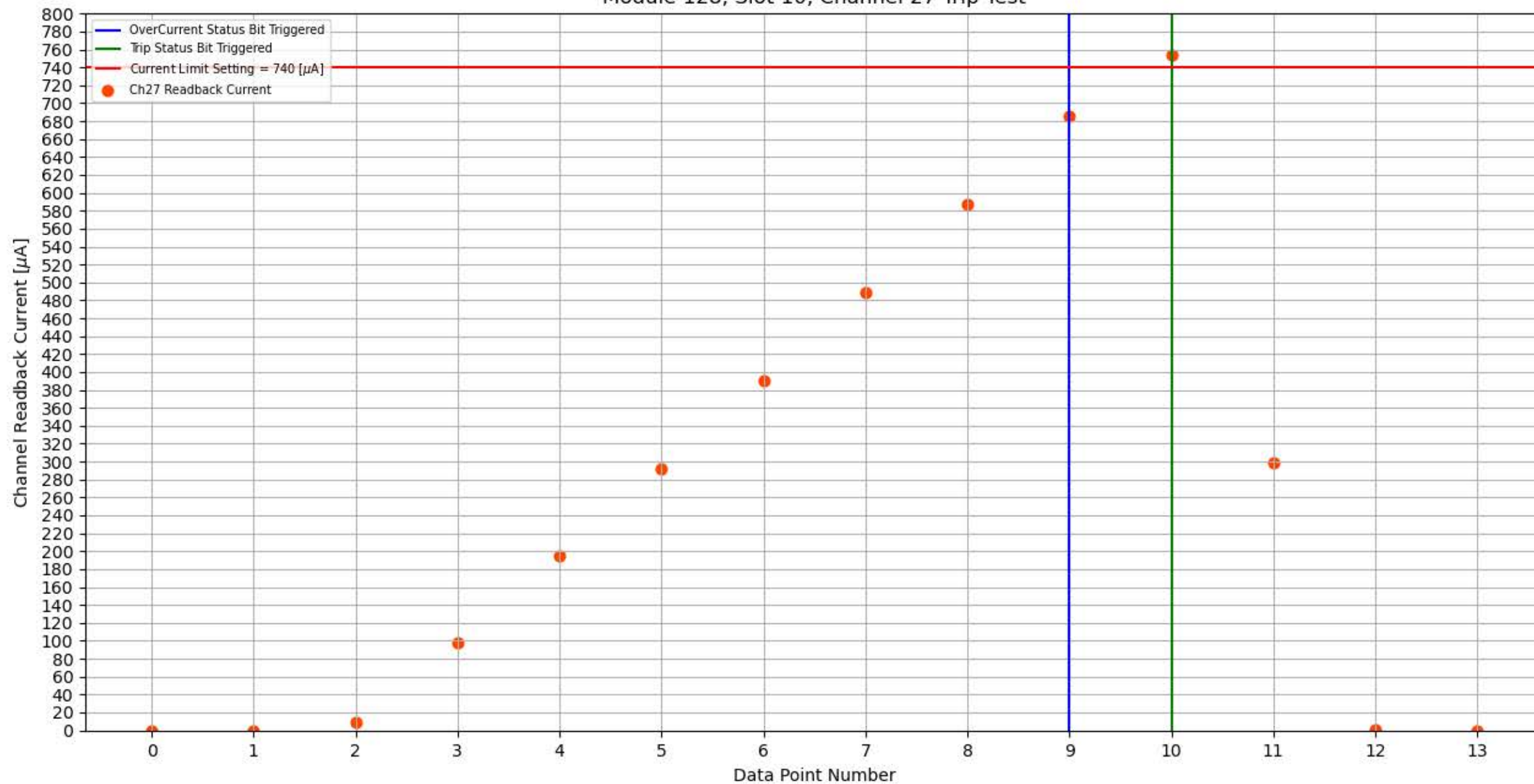
Module 128, Slot 10, Channel 27 Trip Test
