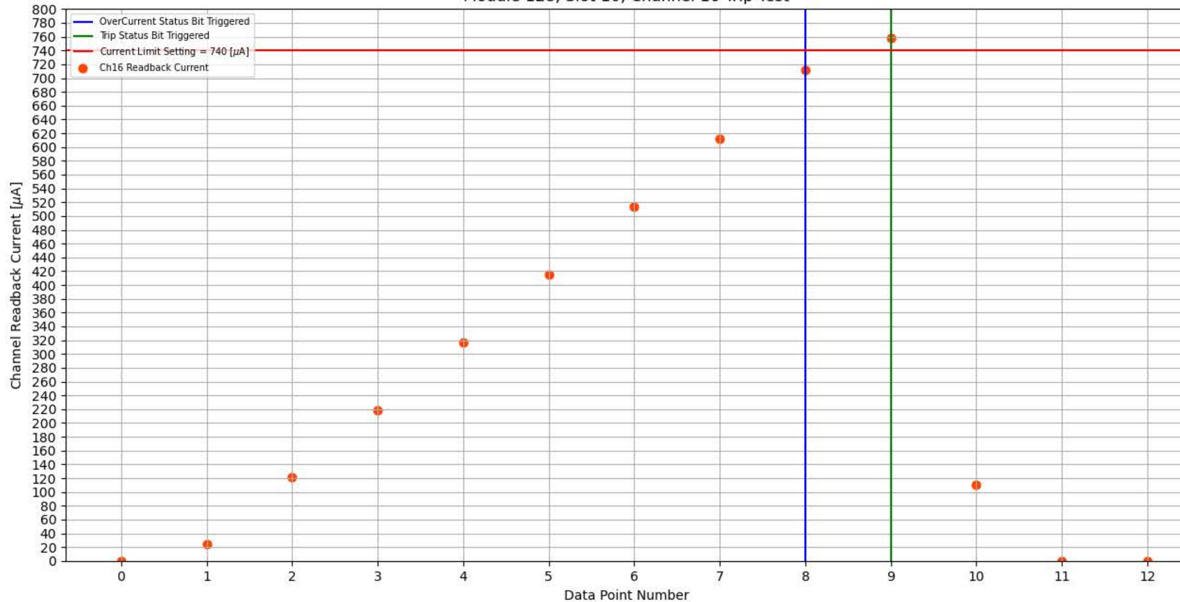
Module 128, Slot 10, Channel 16 Trip Test
