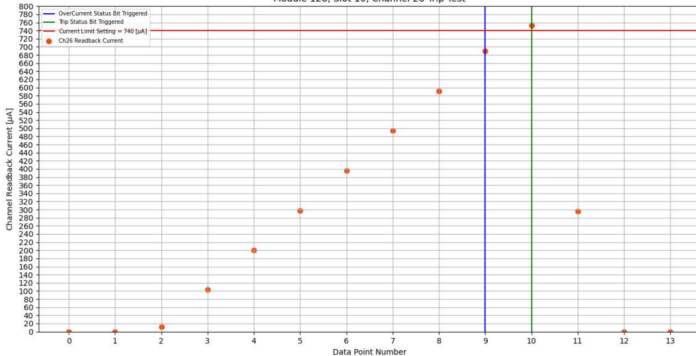
Module 128, Slot 10, Channel 26 Trip Test
