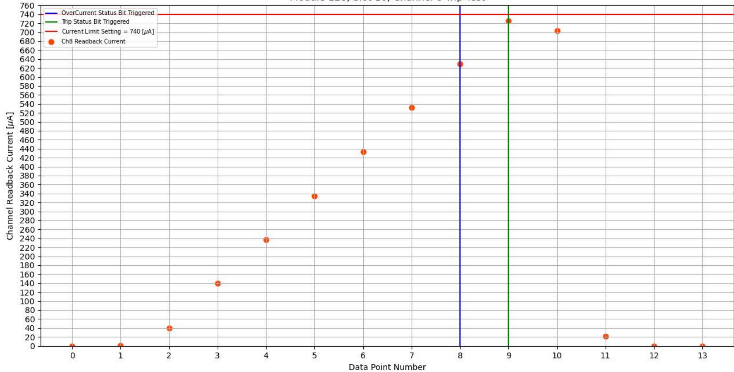
Module 128, Slot 10, Channel 8 Trip Test
