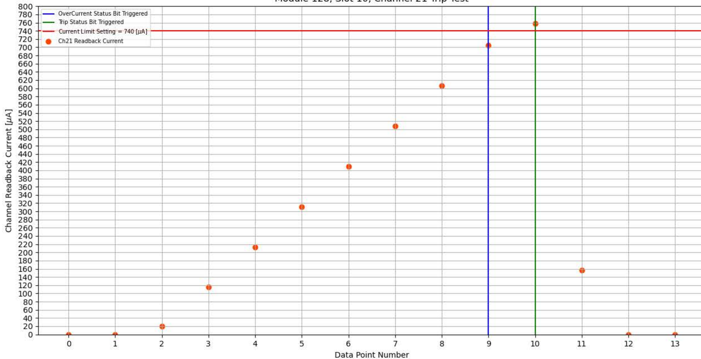
Module 128, Slot 10, Channel 21 Trip Test
