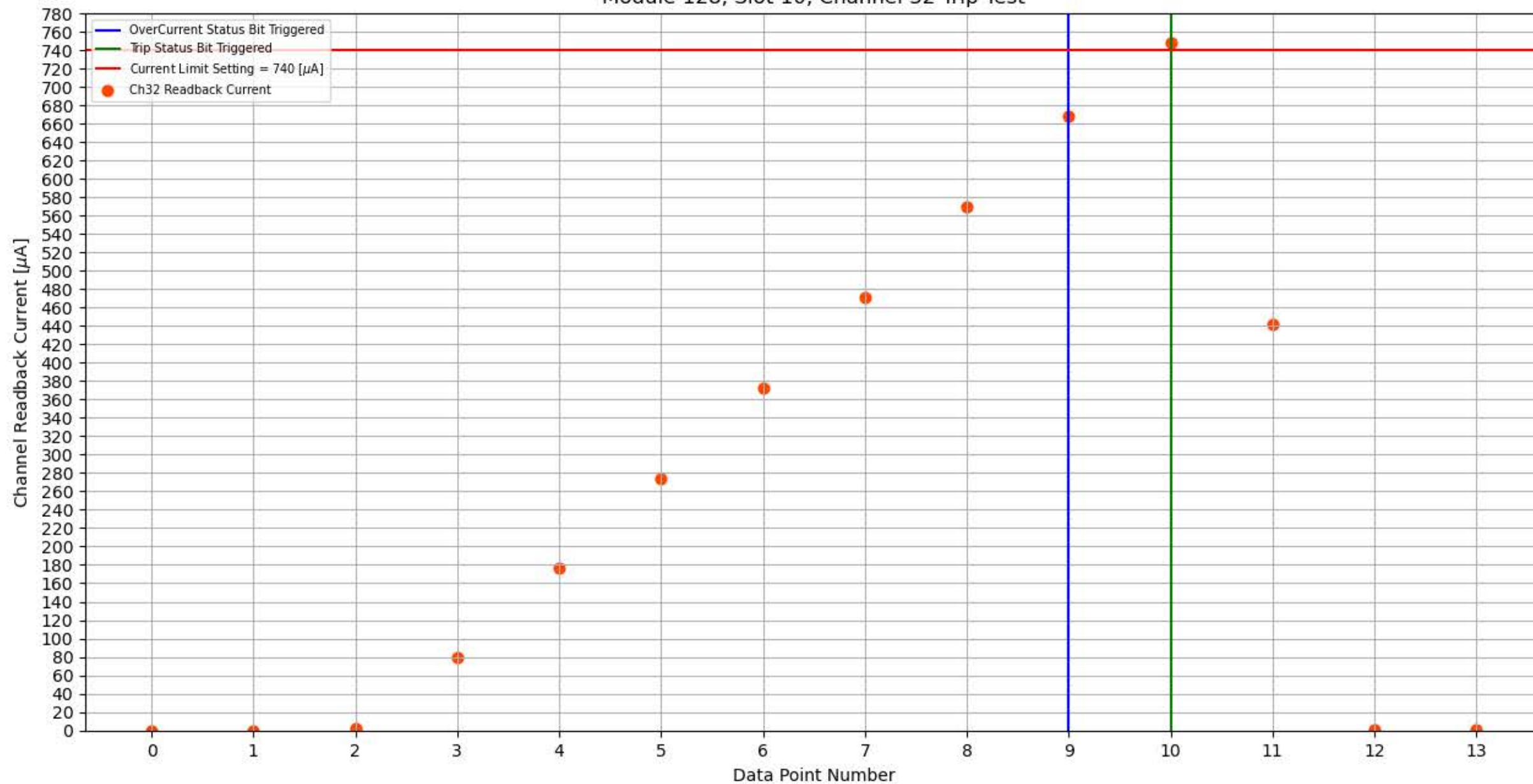
Module 128, Slot 10, Channel 32 Trip Test
