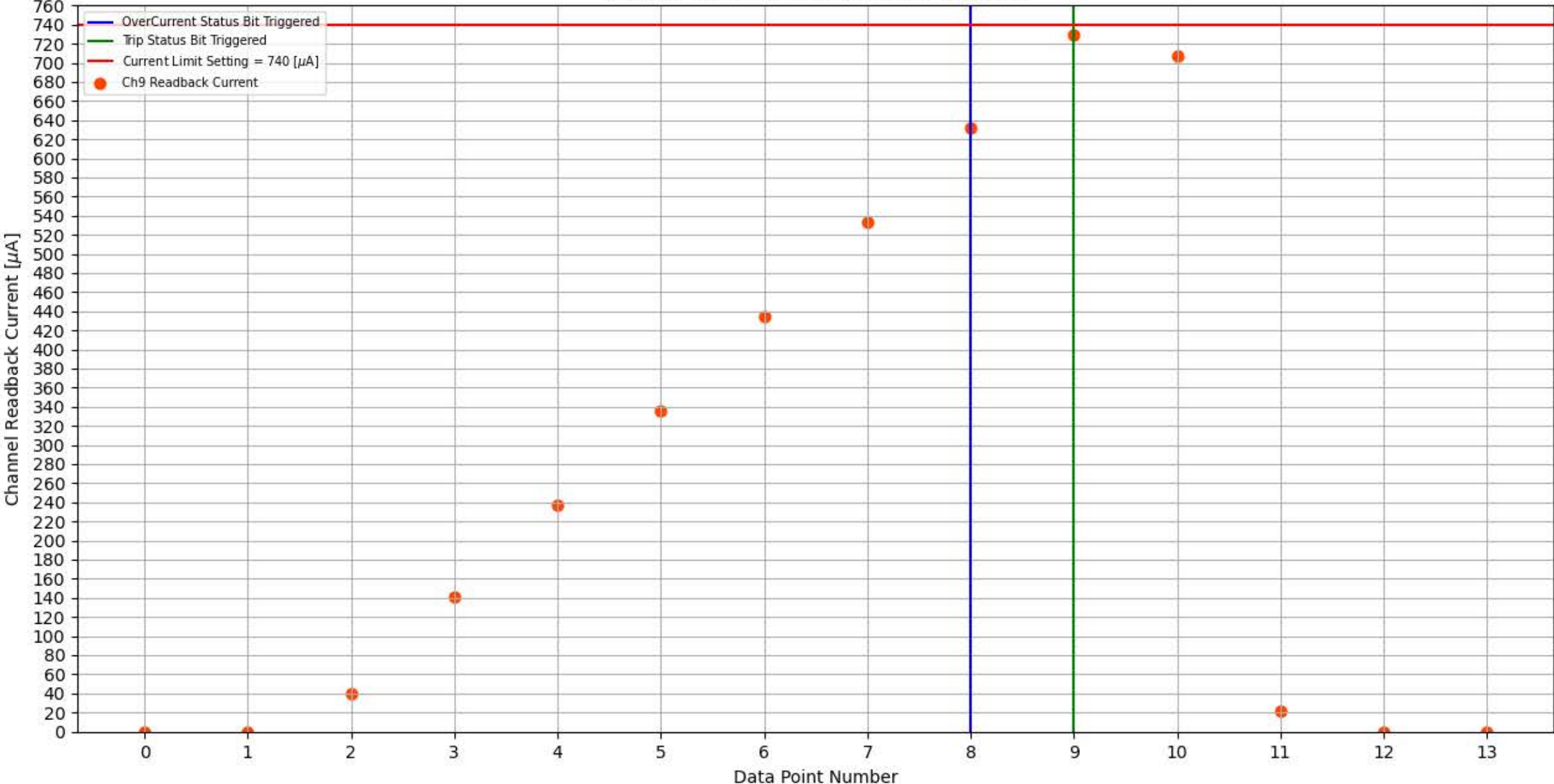
Module 128, Slot 10, Channel 9 Trip Test
