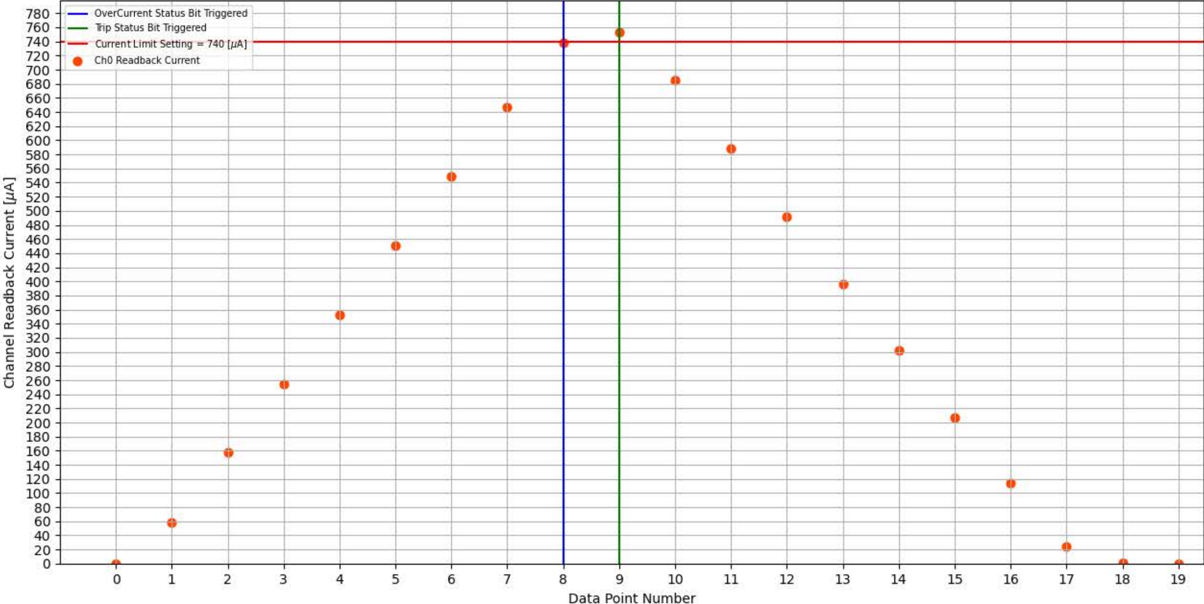
Module 128, Slot 10, Channel 0 Trip Test
