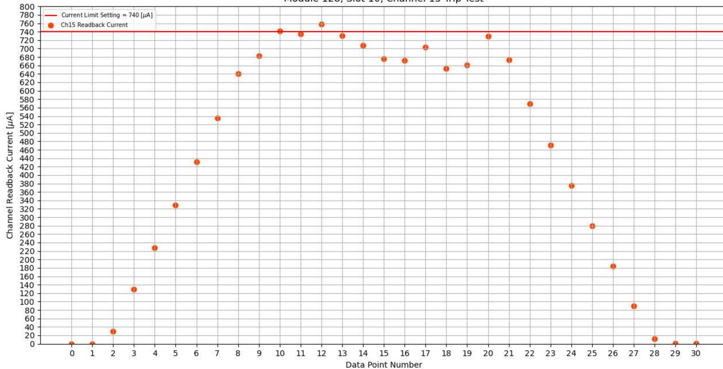
Module 128, Slot 10, Channel 15 Trip Test
