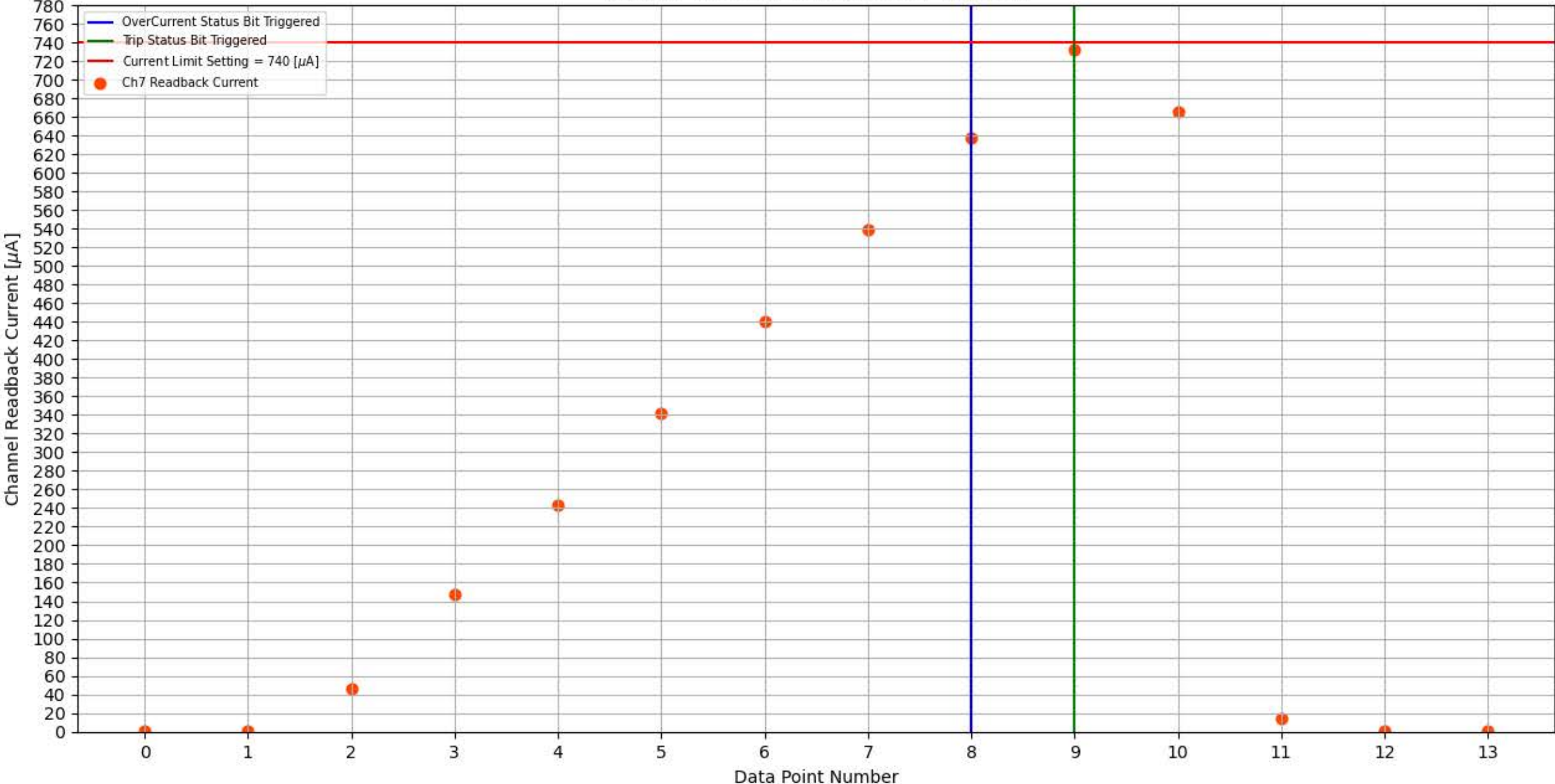
Module 128, Slot 10, Channel 7 Trip Test
