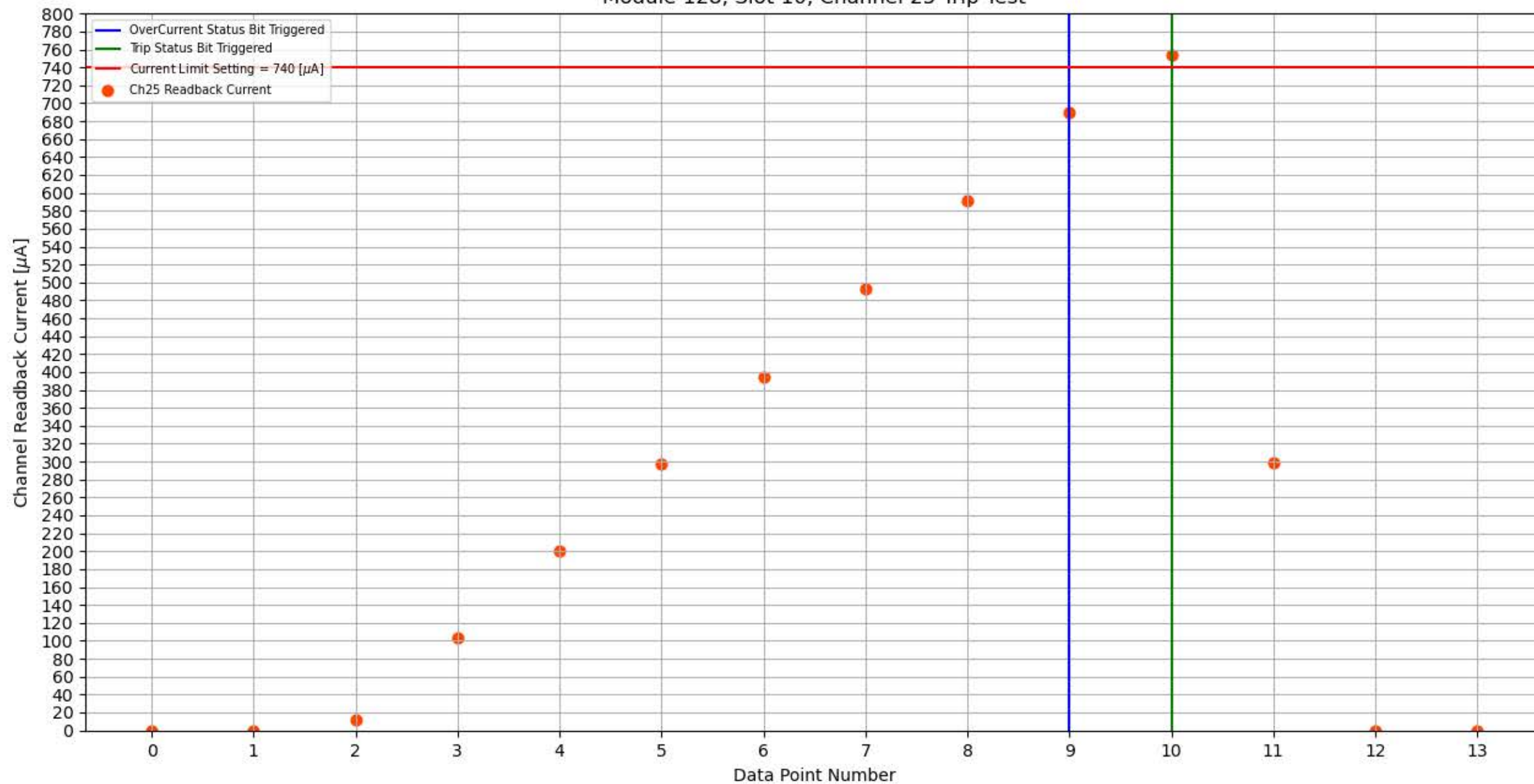
Module 128, Slot 10, Channel 25 Trip Test
