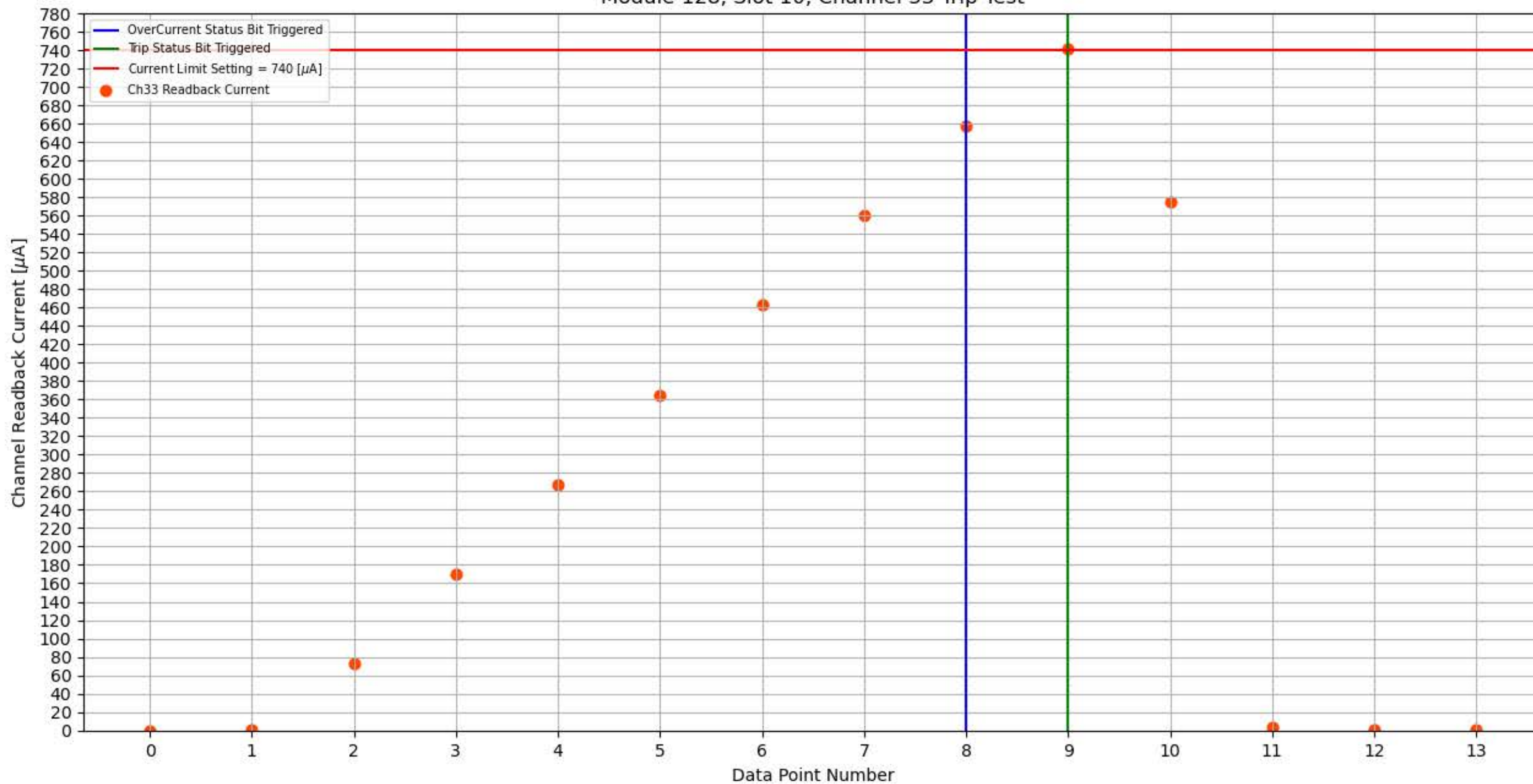
Module 128, Slot 10, Channel 33 Trip Test
