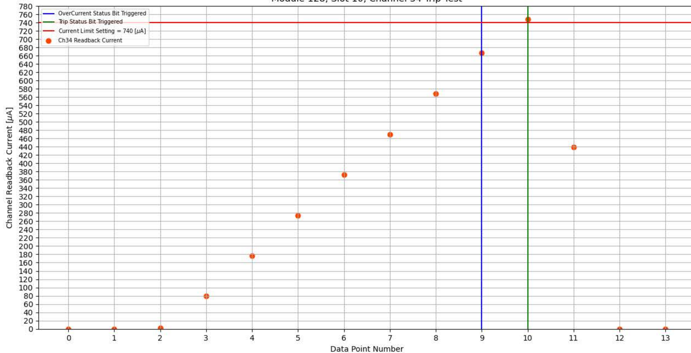
Module 128, Slot 10, Channel 34 Trip Test
