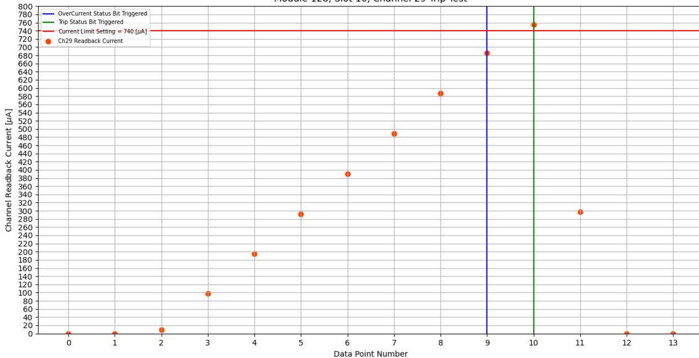
Module 128, Slot 10, Channel 29 Trip Test
