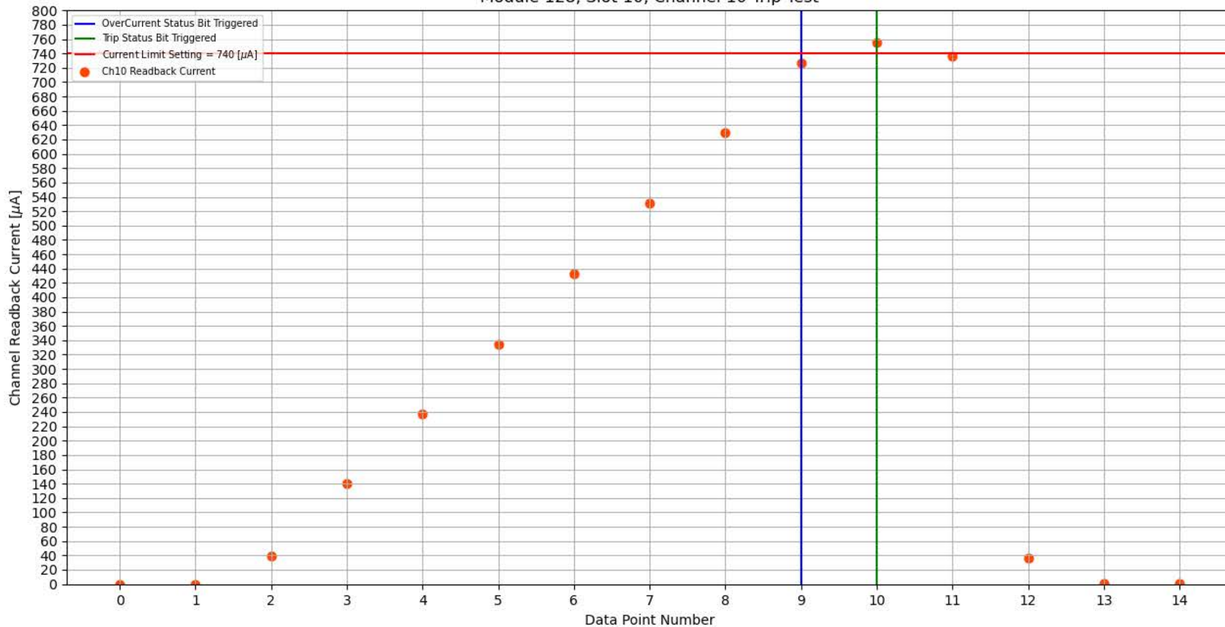
Module 128, Slot 10, Channel 10 Trip Test
