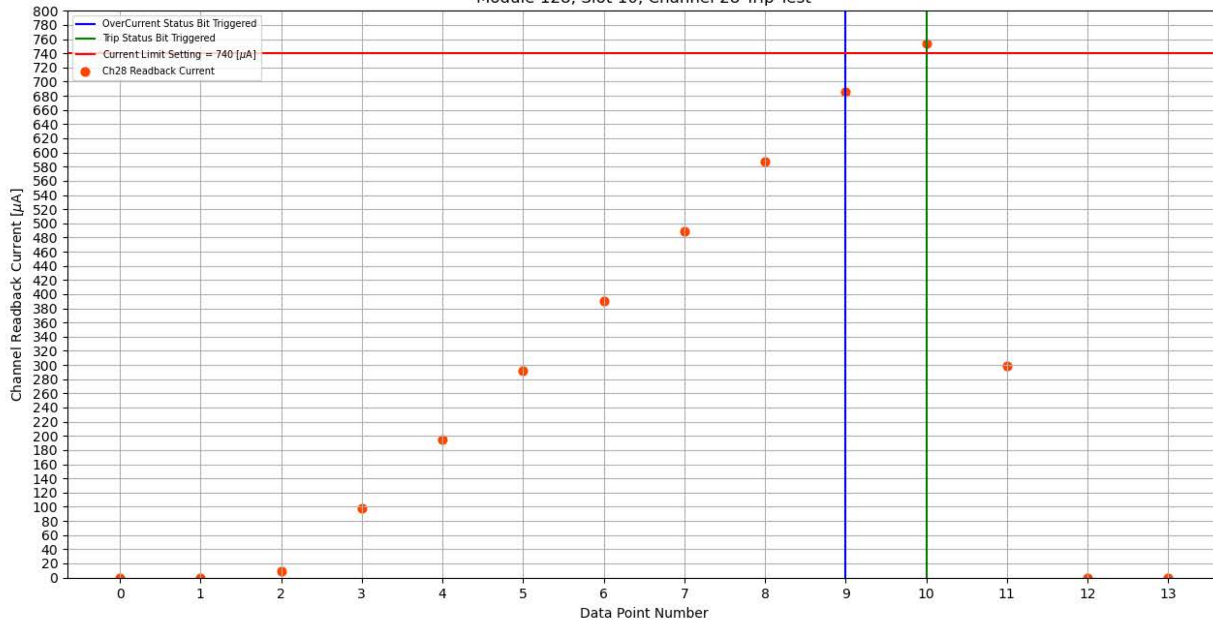
Module 128, Slot 10, Channel 28 Trip Test
