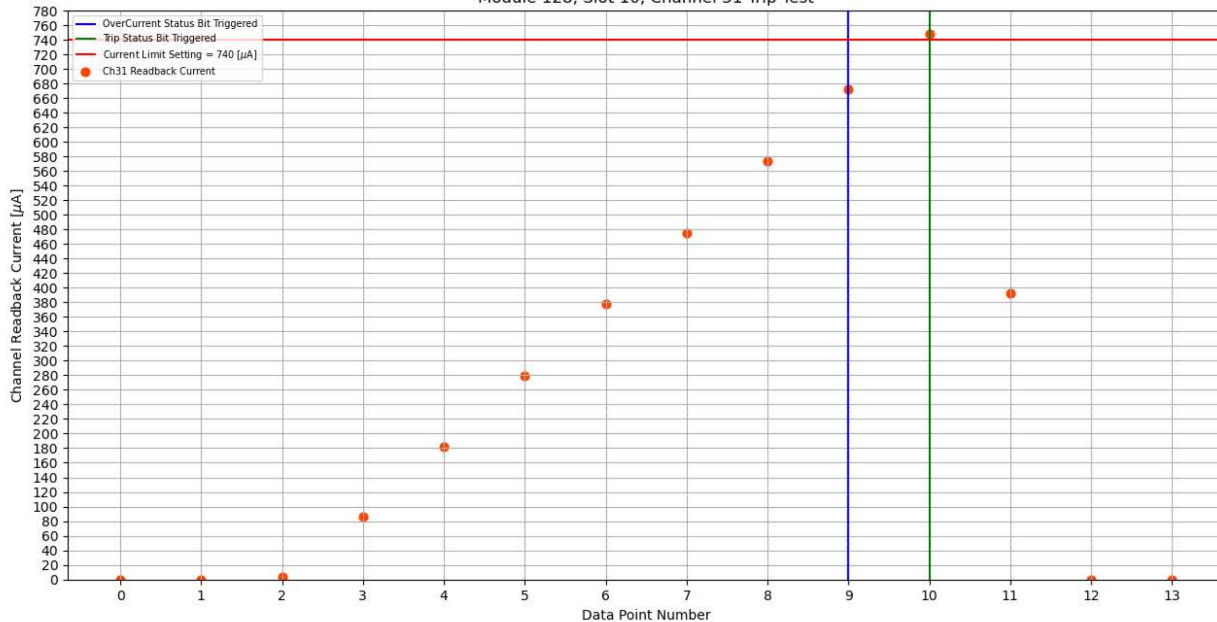
Module 128, Slot 10, Channel 31 Trip Test
