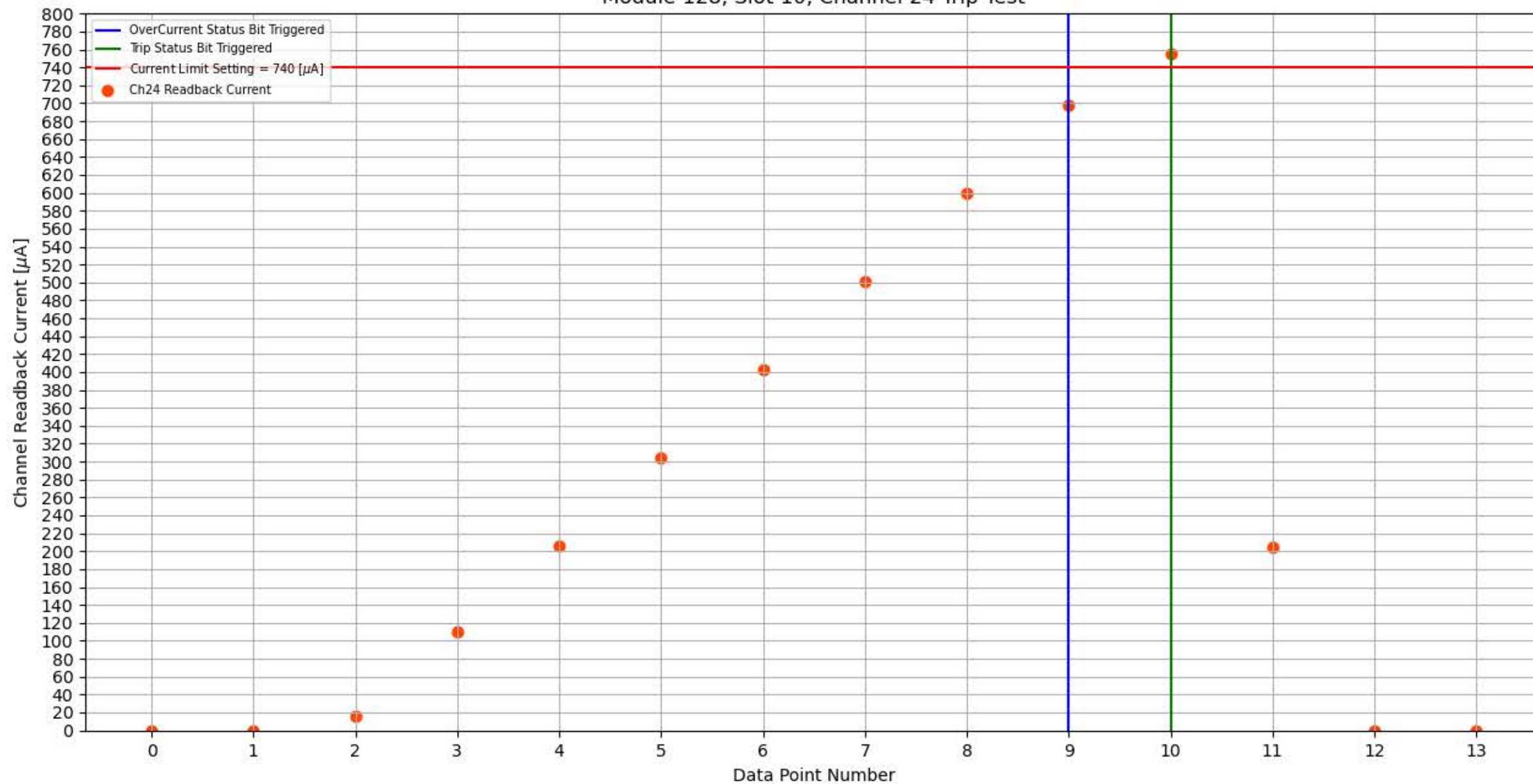
Module 128, Slot 10, Channel 24 Trip Test
