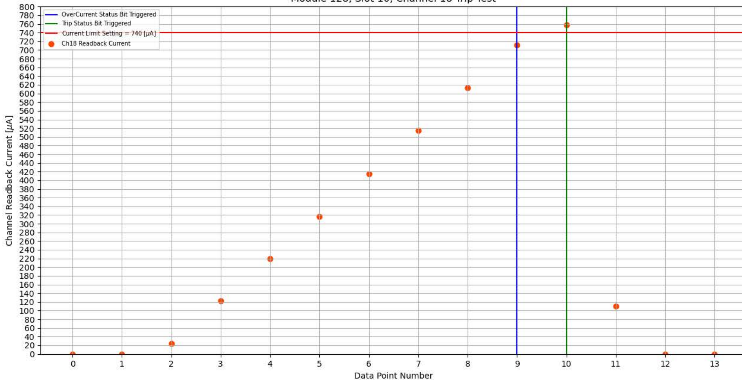
Module 128, Slot 10, Channel 18 Trip Test
