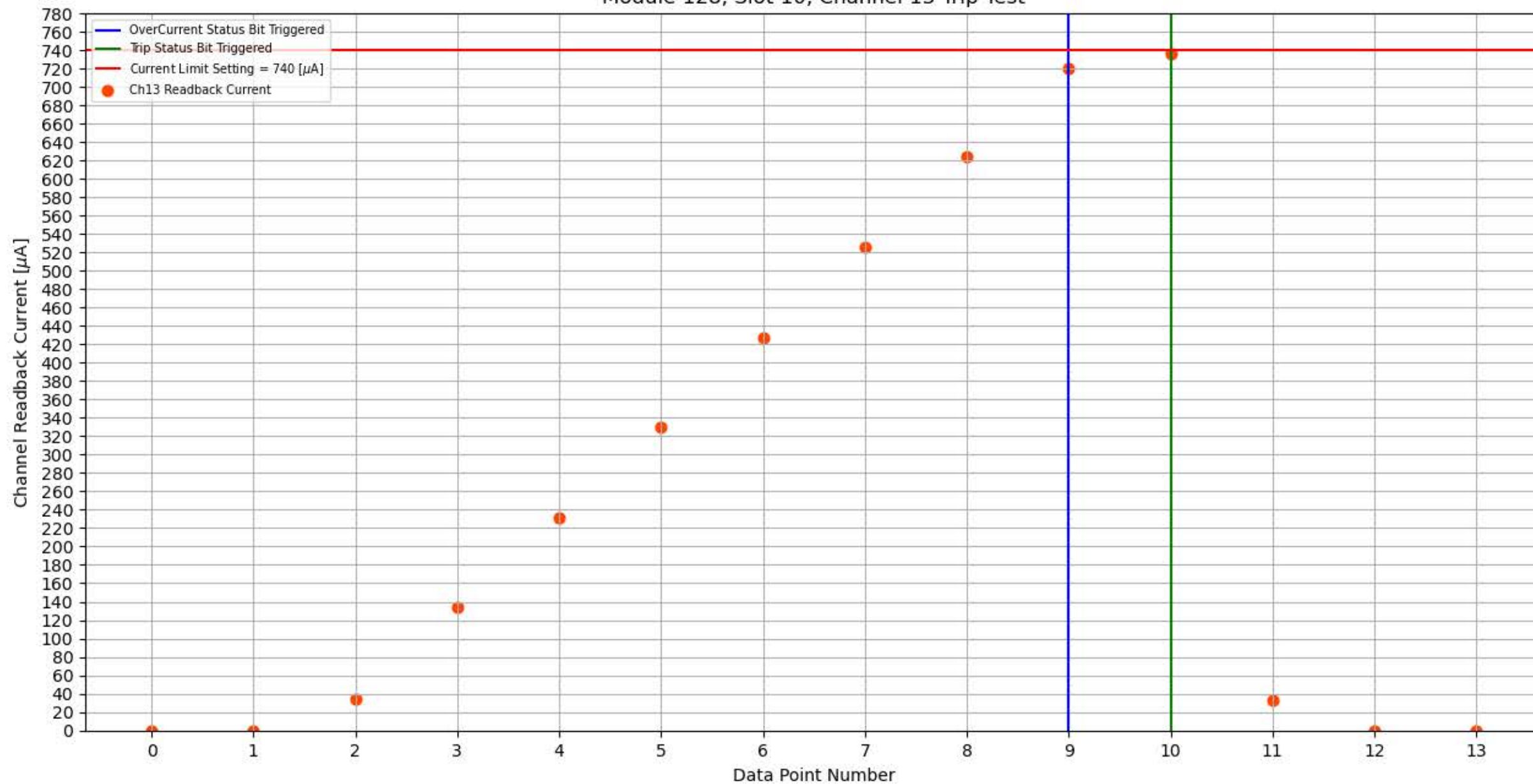
Module 128, Slot 10, Channel 13 Trip Test
