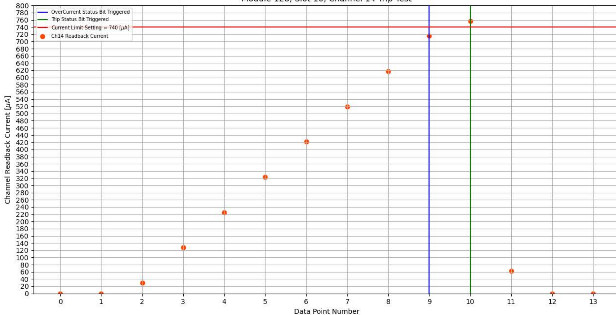
Module 128, Slot 10, Channel 14 Trip Test
