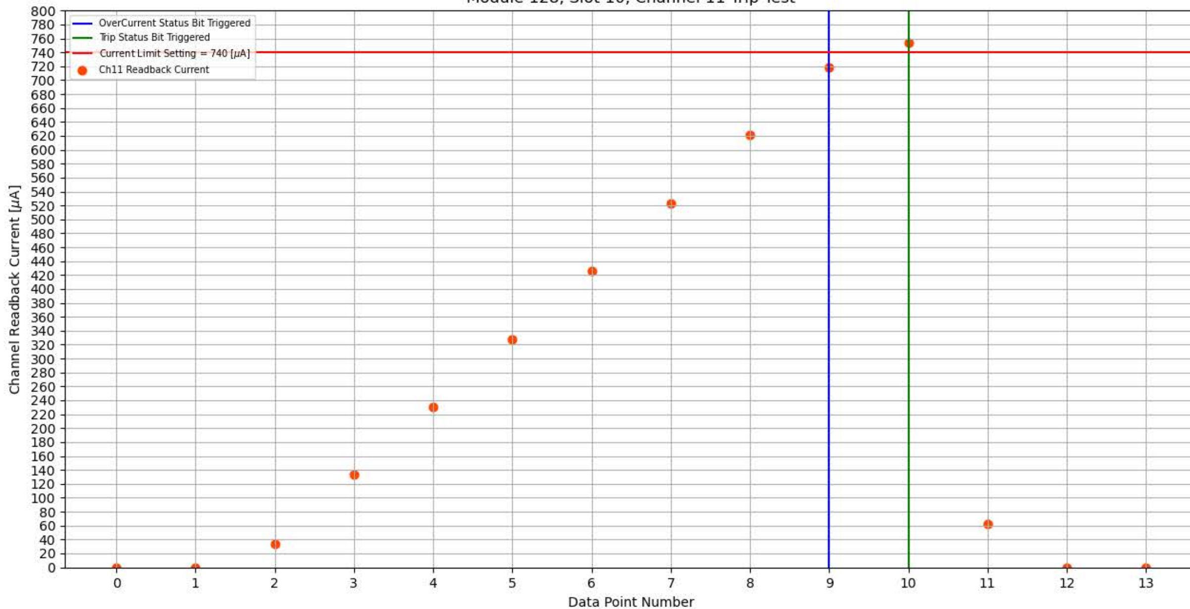
Module 128, Slot 10, Channel 11 Trip Test
