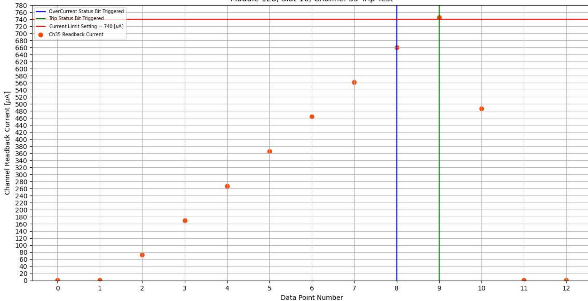
Module 128, Slot 10, Channel 35 Trip Test
