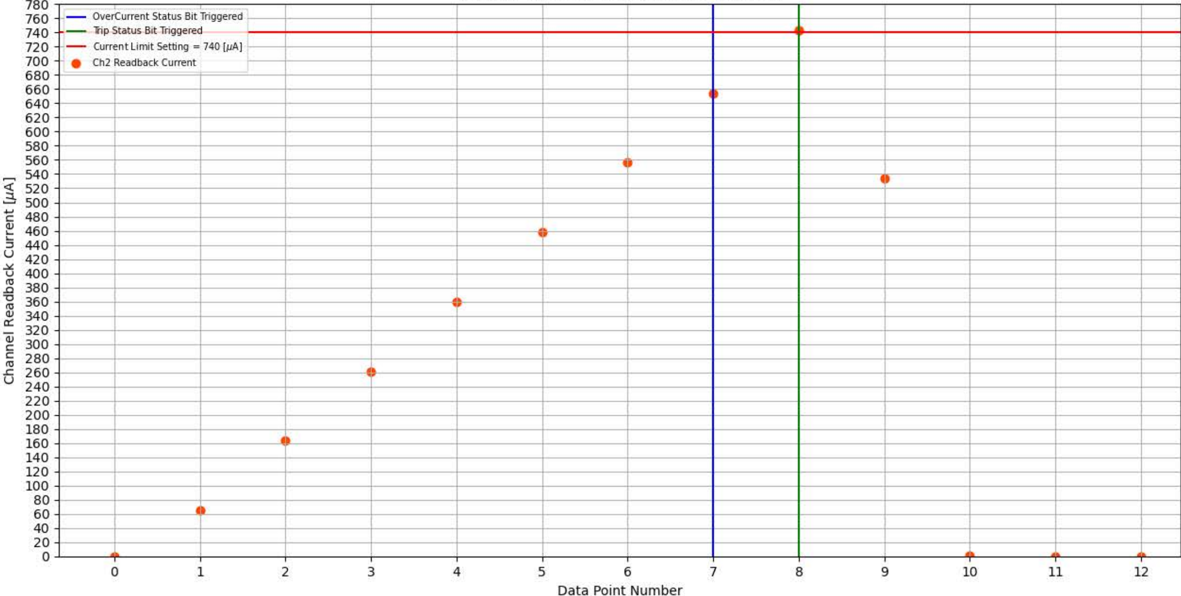
Module 128, Slot 10, Channel 2 Trip Test
