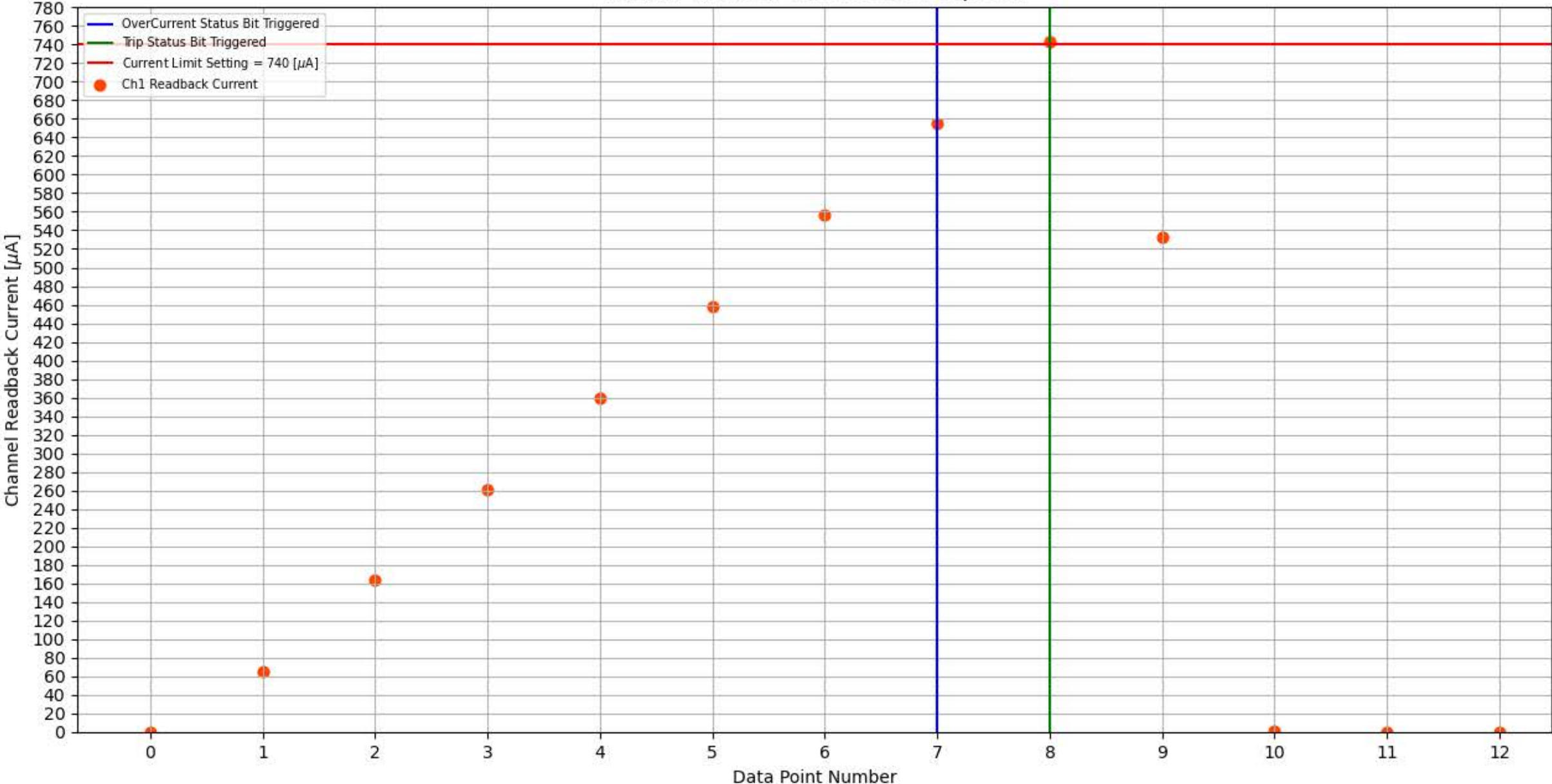
Module 128, Slot 10, Channel 1 Trip Test
