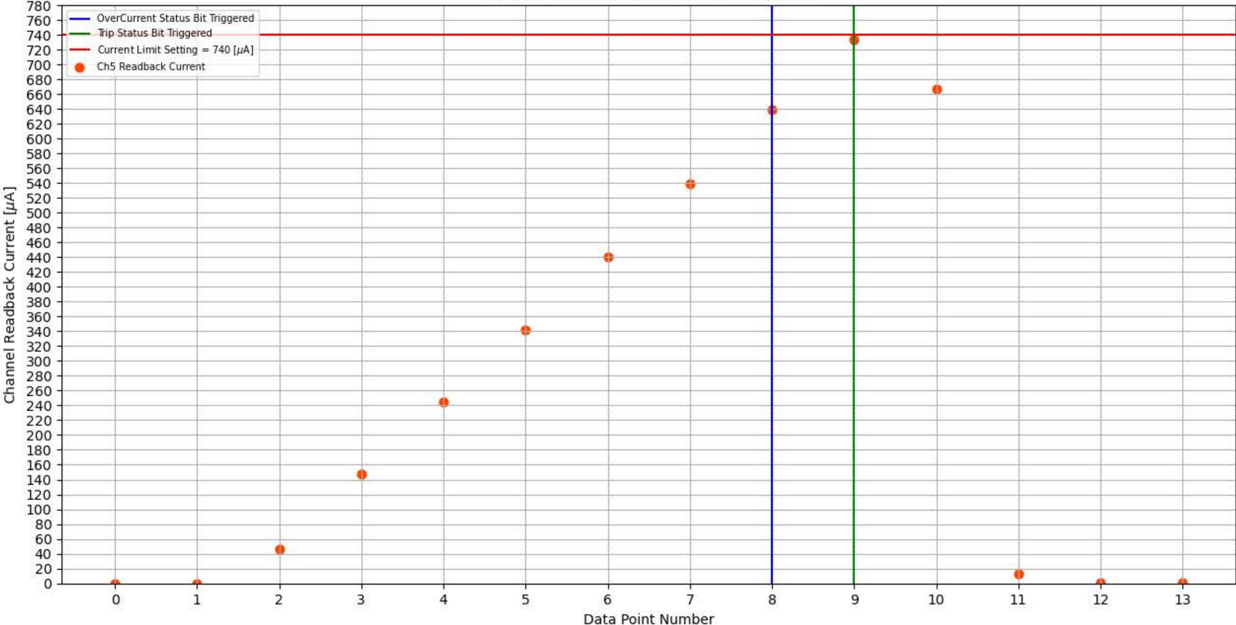
Module 128, Slot 10, Channel 5 Trip Test
