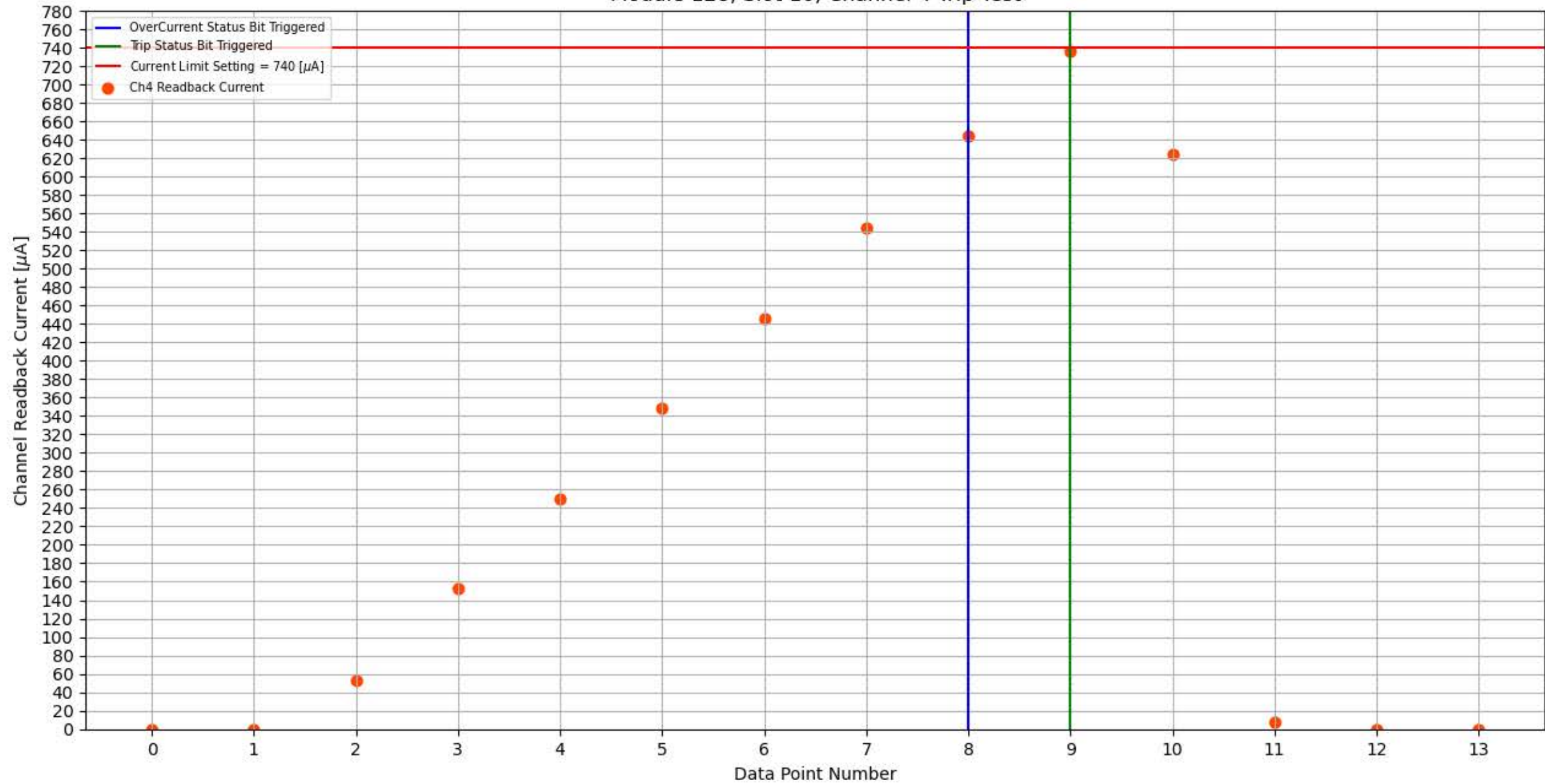
Module 128, Slot 10, Channel 4 Trip Test
