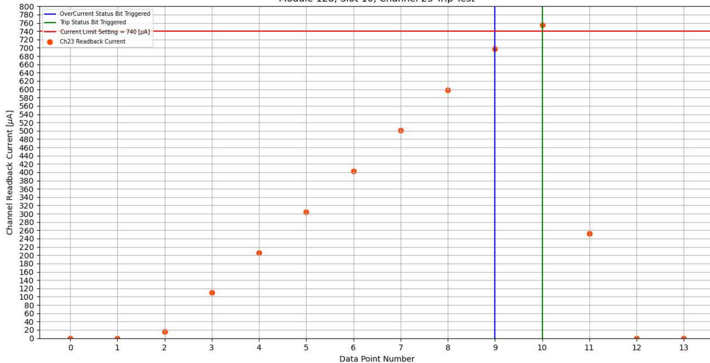
Module 128, Slot 10, Channel 23 Trip Test
