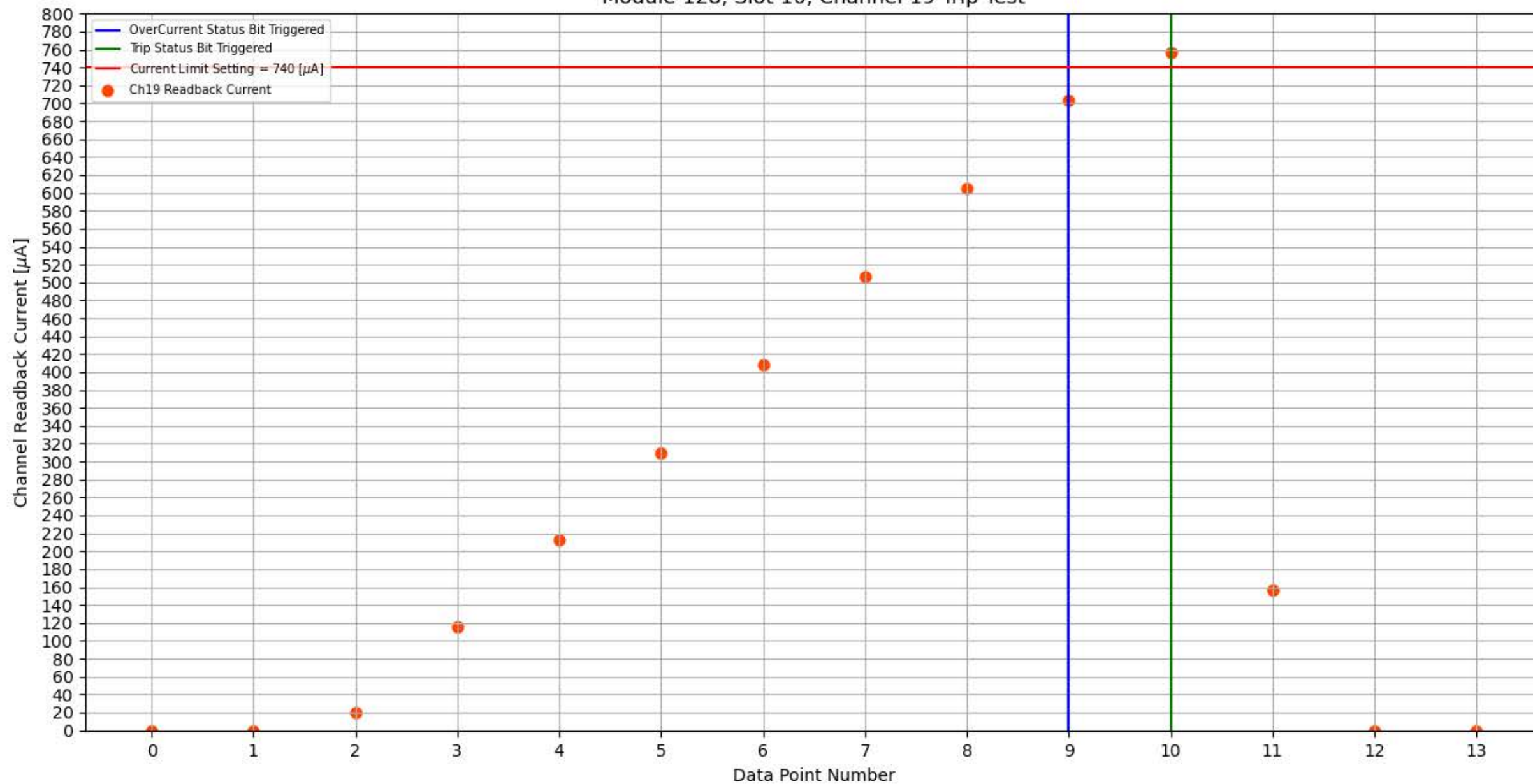
Module 128, Slot 10, Channel 19 Trip Test
