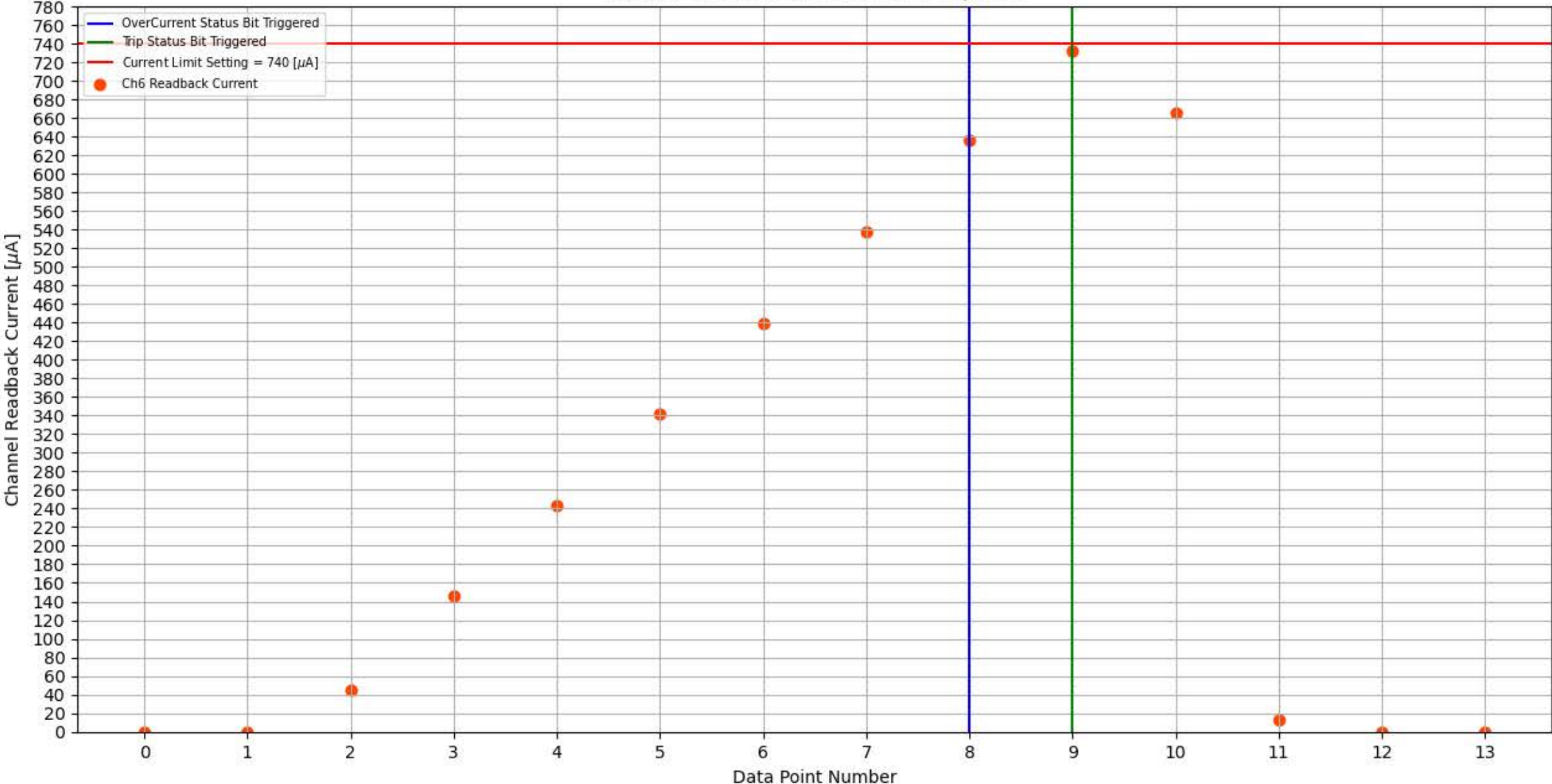
Module 128, Slot 10, Channel 6 Trip Test
