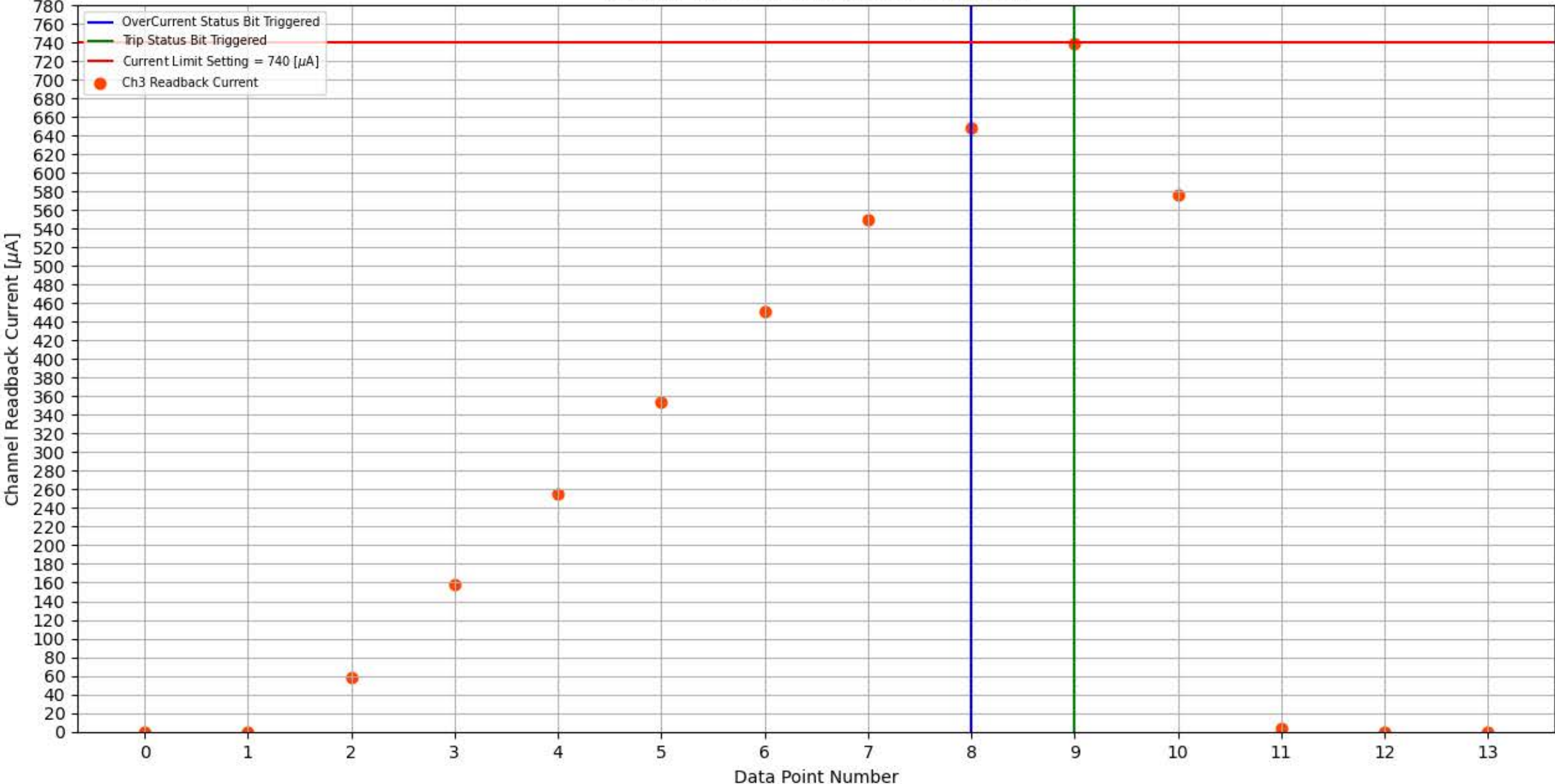
Module 128, Slot 10, Channel 3 Trip Test
