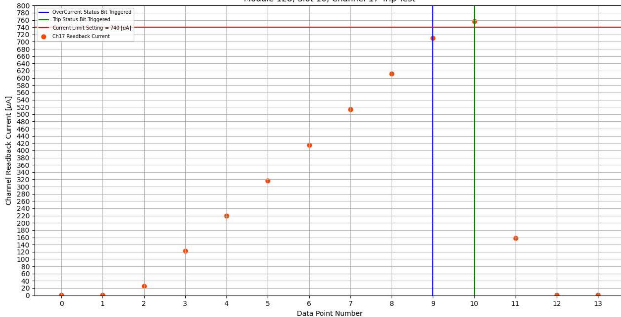
Module 128, Slot 10, Channel 17 Trip Test
